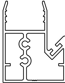
ARA KENET INTERMEDIATE CLAMP Stok : 6 mt 7 mt Ağırlık / Weight: 1,026 Kg/m
