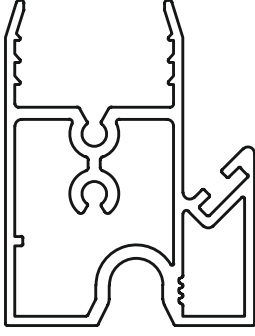
ORTA CAM ALT PROFİL MIDDLE GLASS LOWER PROFILE Stok : 6 mt 7 mt Ağırlık / Weight: 1,026 Kg/m
