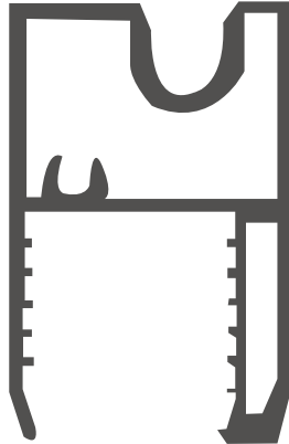
KANAT ALT KENETİ WING LOWER CLAMP Stok : 6 mt 7 mt Ağırlık / Weight: 0,846 Kg/m
