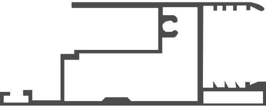
KANAT PROFİLİ WING PROFILE Stok : 6mt 7 mt Ağırlık / Weight: 1,045 Kg/m
