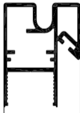
TİJLİ ORTA CAM KENET MEDIUM GLASS SEAM WITH ROD Stok : 7 mt Ağırlık / Weight: 0,883 Kg/m
