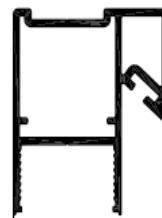
TİJLİ ARA KENET ROD-SHAFT INTERMEDIATE STITCH Stok : 7 mt Ağırlık / Weight: 0,796 Kg/m
