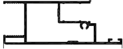
KANAT PROFİLİ WING PROFILE Stok : 7 mt Ağırlık / Weight: 1,004 Kg/m
