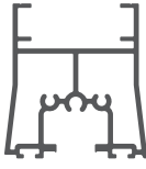
ISICAM BAZA THERMOPANE BASE
